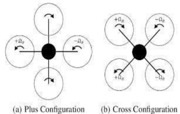
Fig.2 Quadcopter configuration.
