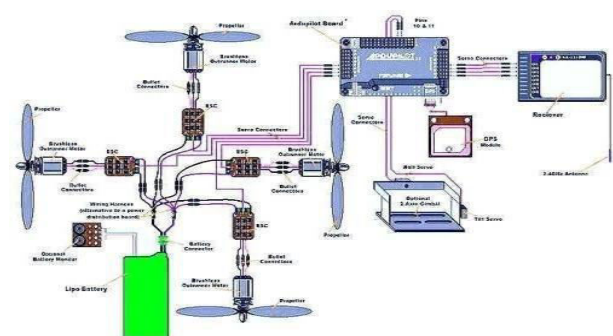
Fig.3 circuit diagram of drone
