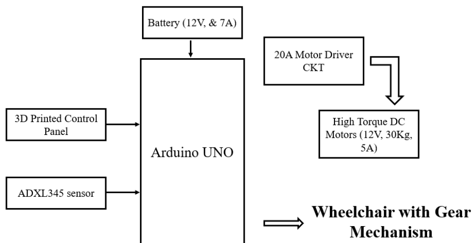
Figure 1: Proposed block diagram of head movement-based real-time wheelchair with gear mechanism.
